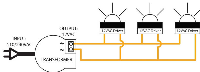
Remote Transformer. Fixture with Internal Driver Wired in Parallel
