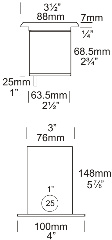
Floor Canister (supplied with luminaire)
